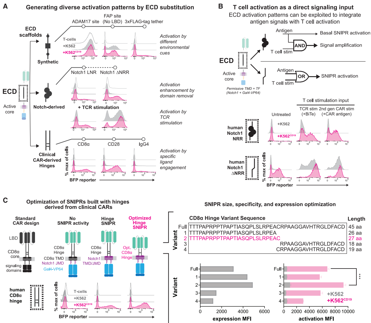
Figure 2. The ECD module defines activation triggers and diversifies sensor functions
