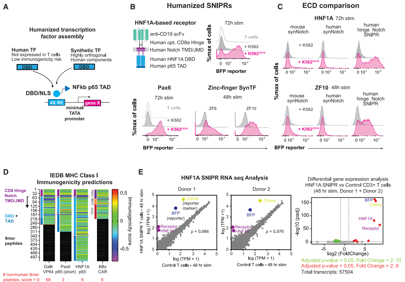
Figure 5. Humanization of SNIPRs to reduce immunogenicity potential for cell-based therapies
