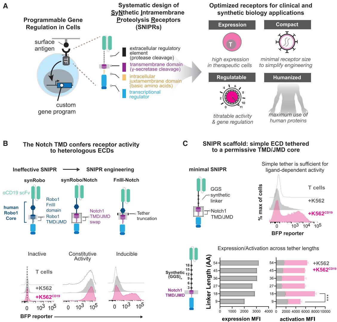
Figure 1. Design of synthetic RIP receptors for customized antigen-dependent gene regulation in therapeutic cells
