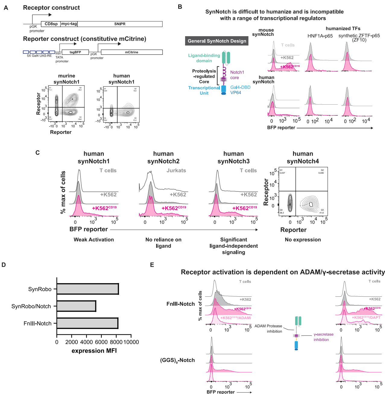
Figure S1. Construct designs, expression of Robo/FnIII receptors, and drug inhibition studies, related to Figure 1
