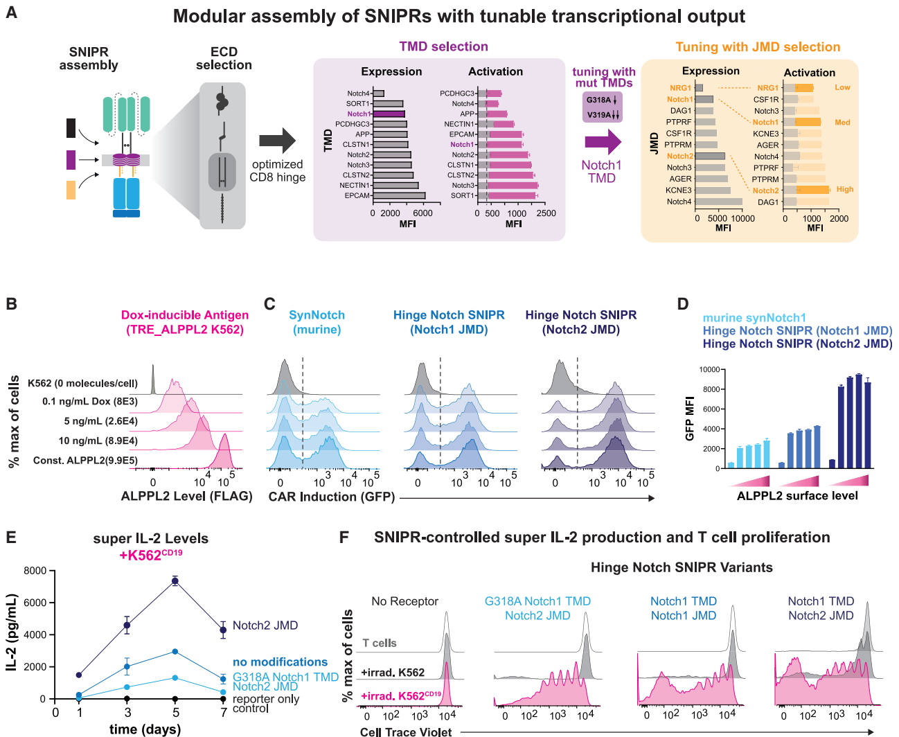
Figure 4. Enhanced sensitivity and tunable gene regulation through SNIPR engineering
