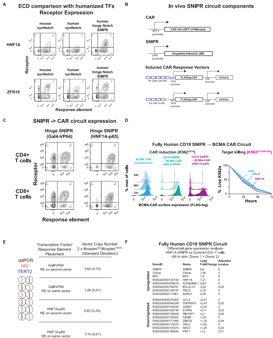
Figure S5. Constructs, expression of humanized and non-humanized receptors, and individual tumor growth curves, related to Figure 5
