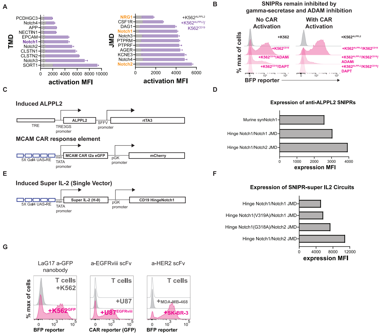
Figure S4. Hinge SNIPR TMD and JMD, drug inhibition studies, construct designs, expression data, testing with additional LBDs, related to Figure 4
